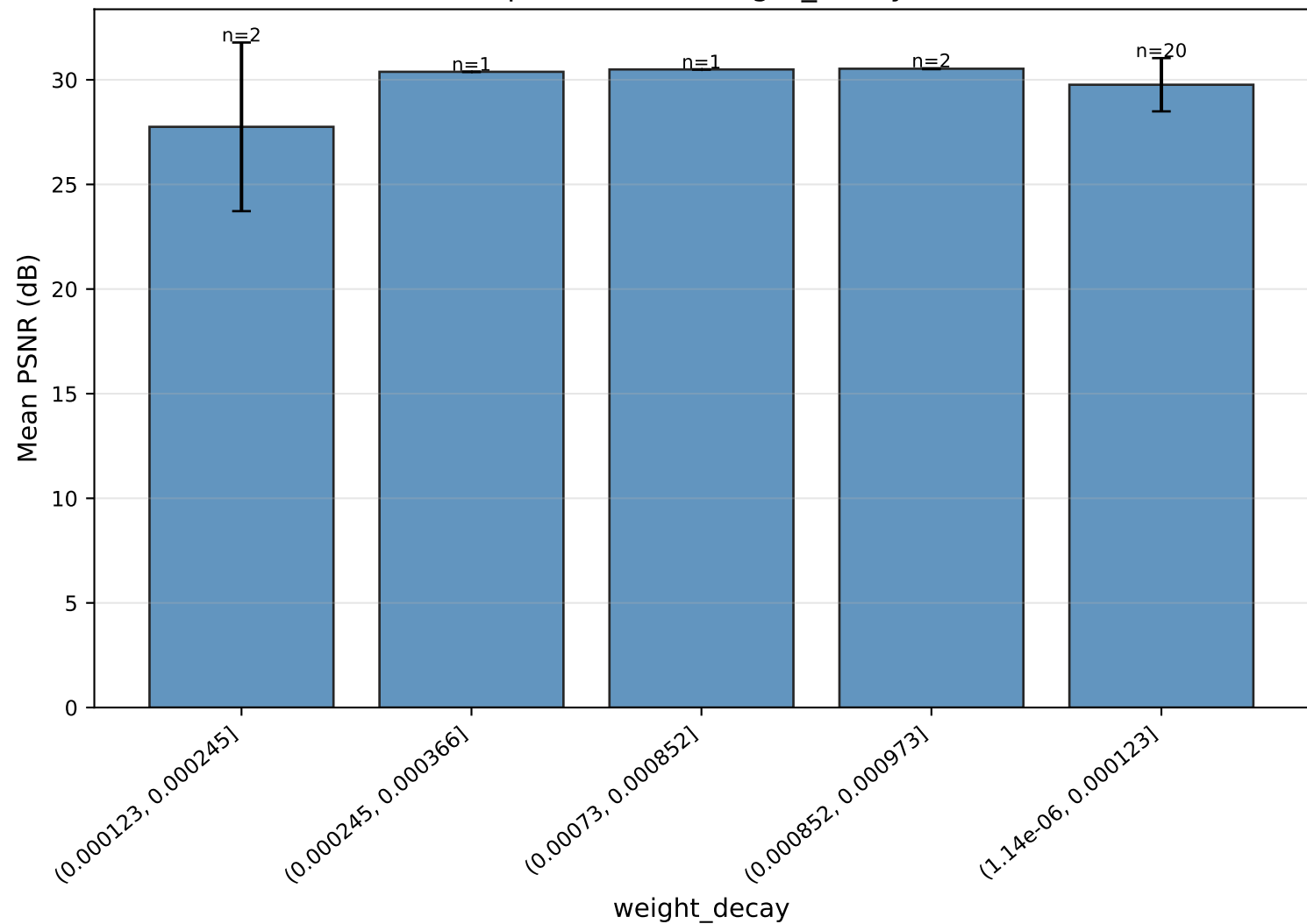
Mean PSNR per value of weight_decay — OmniSR
